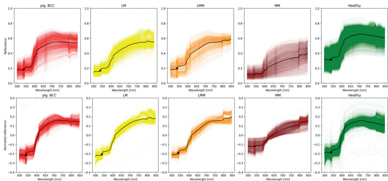
Fig. S3. The difference in the spectra between different lesion types and healthy skin. (a) Reflectance and (b) normalized reflectance. Normalization reduces variance inside each lesion class.
