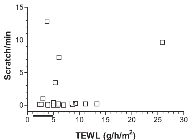
Fig. 3. Correlation between transepidermal water loss (TEWL) and scratching behaviour in 25-week-old scce -transgenic mice. Each open square represents one scce -transgenic mouse; bar = mean and range for TEWL of wild-type littermates ( n=29 ) of the same age.
