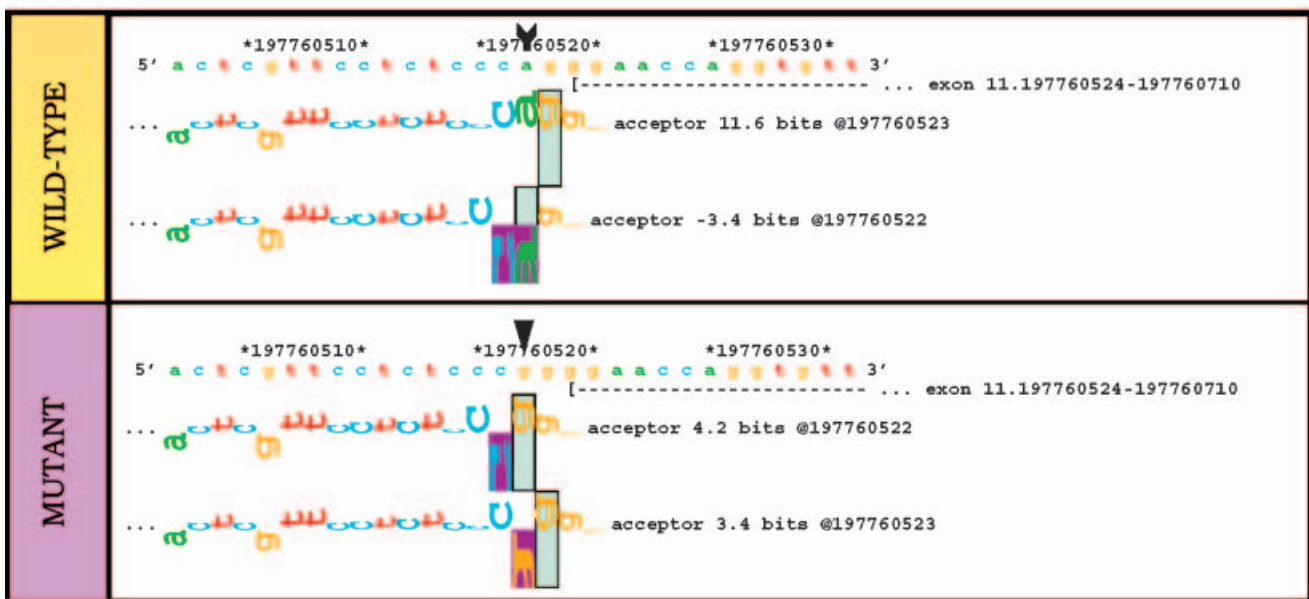
Fig. 1. In silico predictions of cryptic splicing in PKP1 . (A) The c.[1053T>A + 1054+1G>T] mutation abolishes the natural intron 5 donor splice site, with R_i decreased from 6.2 to 0.6 bits. This is predicted to result in intron 5 retention or exon 5 skipping. (B) In contrast, the IVS10-2A>G mutation results in a 'leaky' intron 10 acceptor splice site, with R_i reduced from 11.6 to 3.4 bits. However, this substitution also creates a new cryptic splice site at the last nucleotide of intron 10, with R_i increased from -3.4 to 4.2 bits (c and d). This predicts two outcomes for the mutation IVS10-2A>G: either reduced normal splicing of exon 11, or insertion of an additional single G into the beginning of exon 11 in the mRNA which would lead to a frameshift and downstream premature stop codon.
