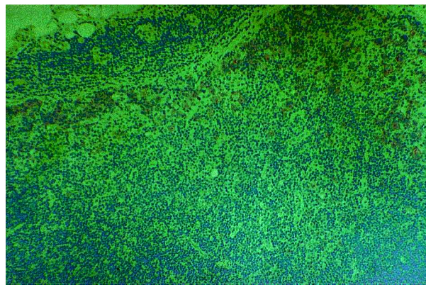
Fig. 3. Histopathology of the sentinel lymph node immunostained for the CD30-antigen. Original magnification: \times 200 .
