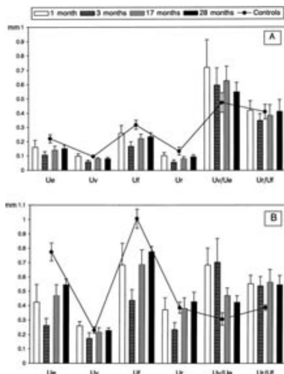
Fig. 2. Skin mechanical parameters in scleredema of Buschke and controls measured by a 2 mm-diameter probe (A) and an 8 mm-diameter probe (B). The average values and 95% confidence intervals are shown.
