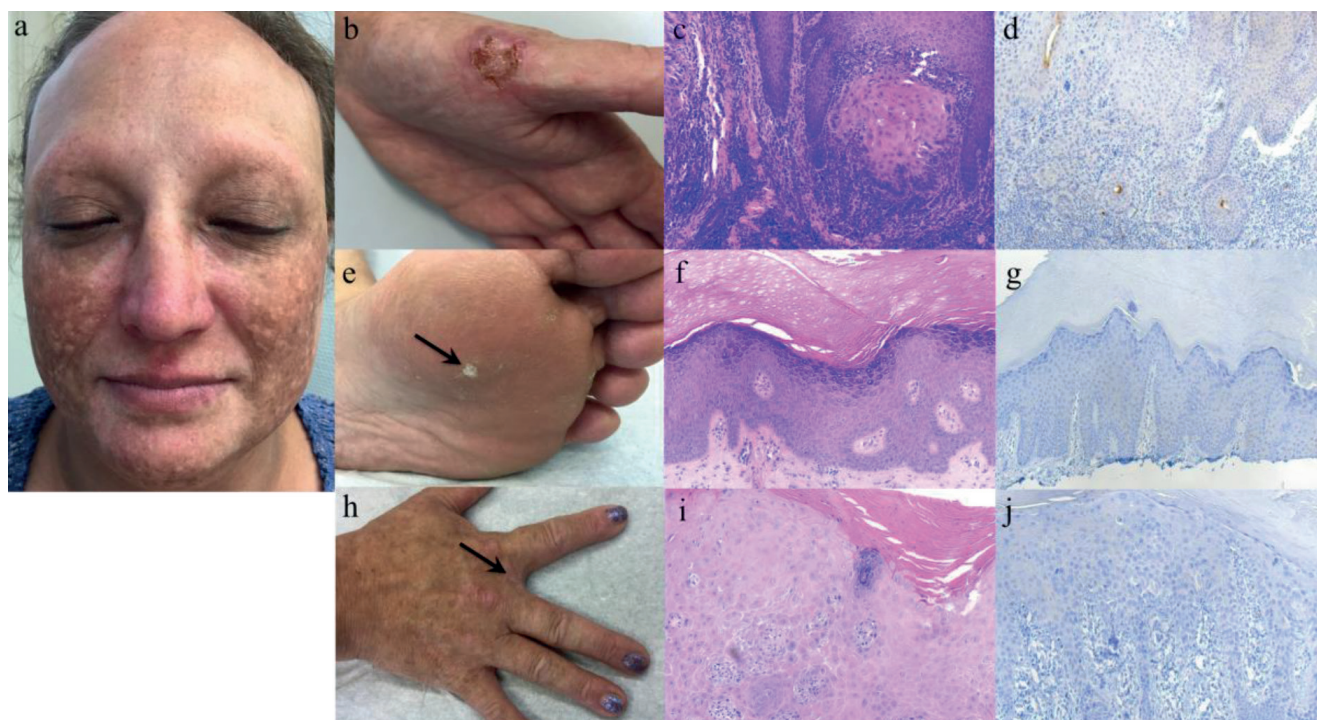
Fig. S4. Clinical presentation at the age of 41 years. (a) Progressive loss of scalp hair. (b) erythematous, erosive plaque on the left thumb. (c) Histopathological analysis demonstrated a well-differentiated, verrucous squamous cell carcinoma. The maximal depth of penetration is 2.6 mm (haematoxylin-eosin staining, original magnification \times 100 ). (d) Negative p16 INK4a -staining (p16 INK4a , original magnification \times 100 ). (e) Presentation of a plantar wart ( black arrow ) located at the left foot and (h) flat verrucae vulgares on the dorsal right hands ( black arrow ). (f, i) Histopathological analysis shows typical features of common warts with hyperpapillomatosis, acanthosis, and parakeratosis (haematoxylin-eosin staining, original magnification \times 100 ) and negative (g, j) p16 INK4a -staining (original magnification \times 100 ).
