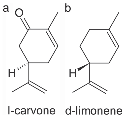
Fig. S1. Representation of chemical structures of: (a) l-carvone and (b) d-limonene.
