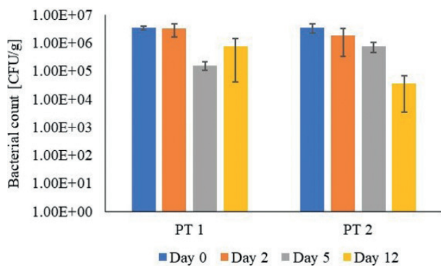
Fig. S2. Short-term stability of the bacterial gel stored at room temperature over 12 days. Data are presented as mean \pm standard deviation (SD). CFU: colony-forming unit; PT1: probiotic topical 1; PT2: probiotic topical 2.
