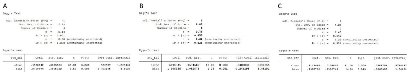
Fig. S3. SuppInfo Egger's test and Begg's test of the studies included in depression (A), anxiety (B) and suicidal ideation/ self-harm (C)
