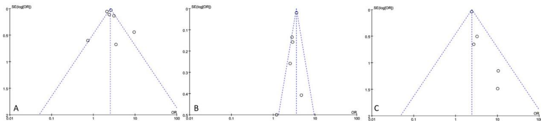
Fig. S2. SuppInfo The funnel plot of the studies included in depression (N=8), anxiety (N=6) and suicidal ideation/ self-harm (N=5)
