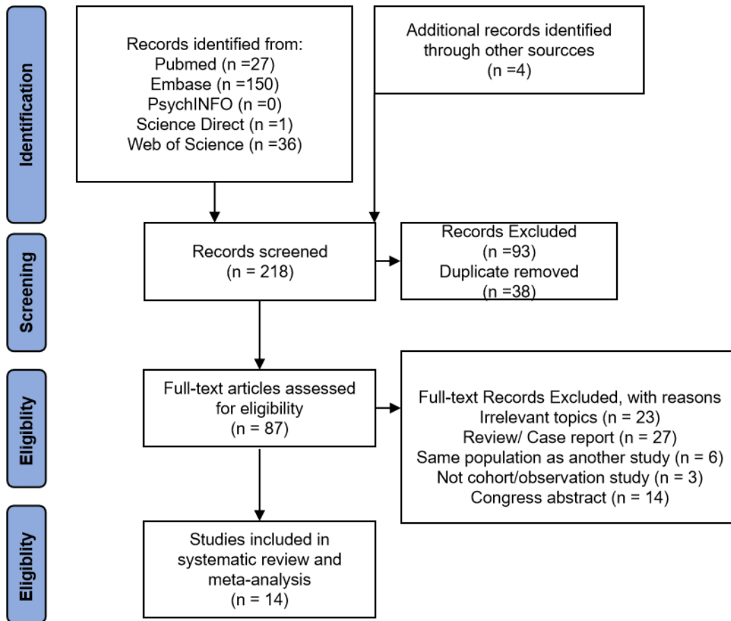
Fig. S1. PRISM flow diagram of study inclusion
