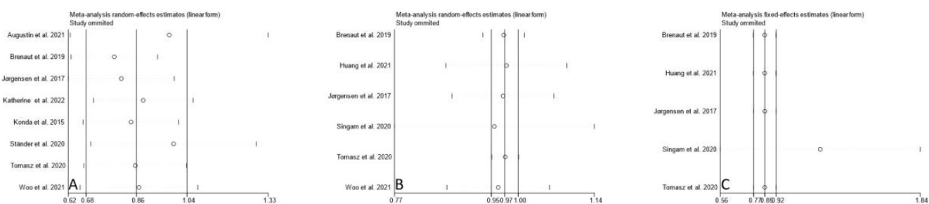
Fig. S4. SuppInfo one-by-one elimination method of the studies included in depression (A), anxiety (B) and suicidal ideation/ self-harm (C)
