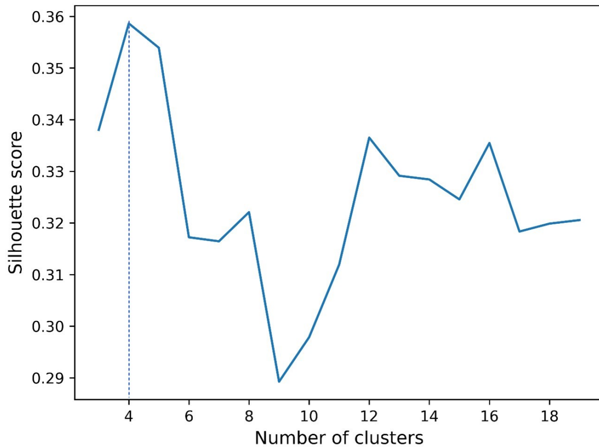
Fig. S1. Silhouette plot showing optimal number of clusters
