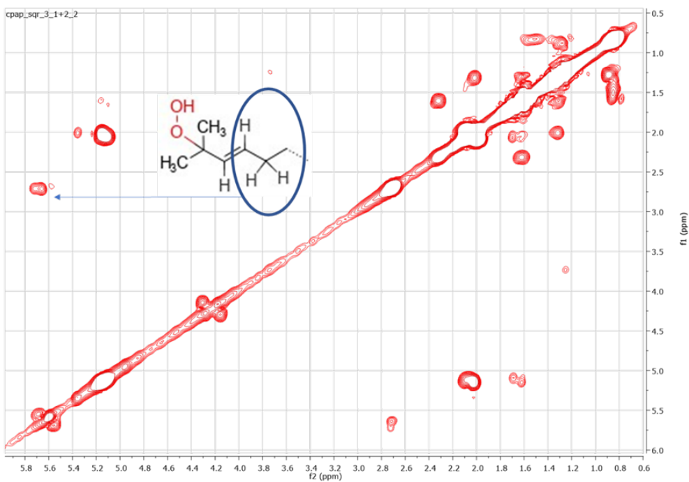
Fig. S2. COSY spectrum of SQ and 2-SQOOH in CDCl 3
