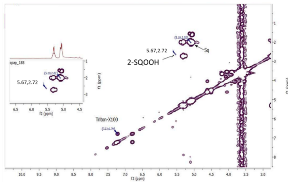
Fig. S3. COSY spectrum ( \text{CDCl}_3 ) of the control culture with linoleic acid and SQ but without M. restricta . A negligible amount of 2-SQOOH was observed by the presence of minor cross-peaks at 5.67/2.72.
