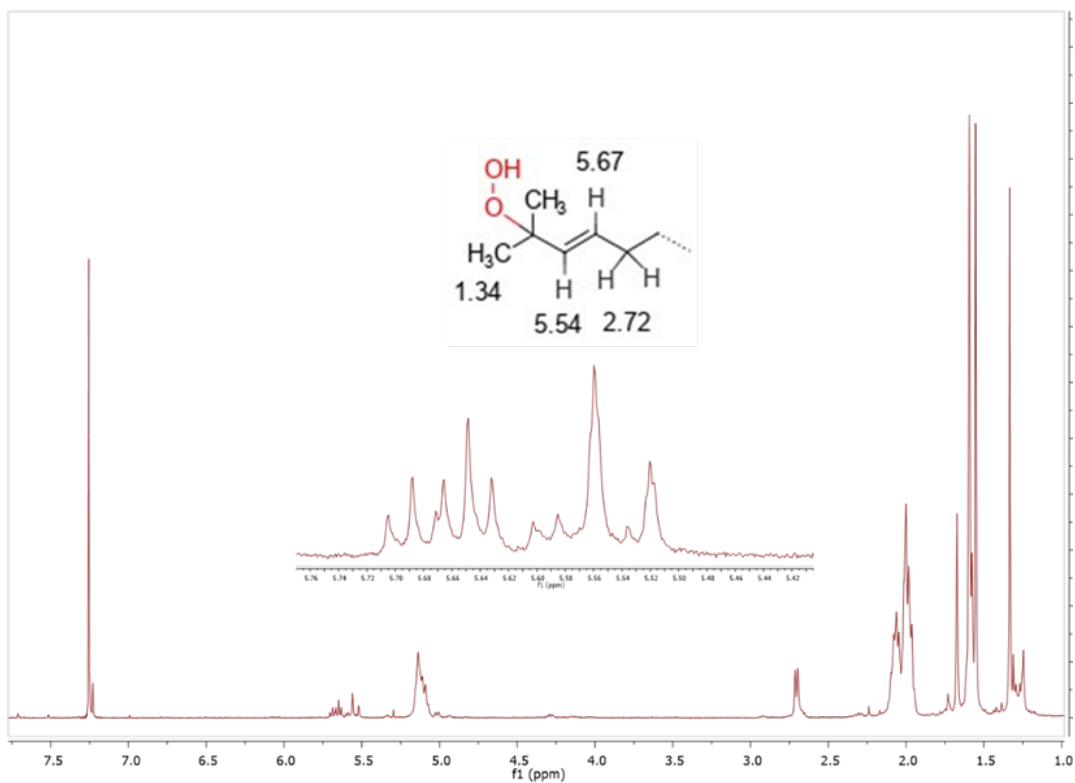
Fig. S2. COSY spectrum of SQ and 2-SQOOH in CDCl 3
