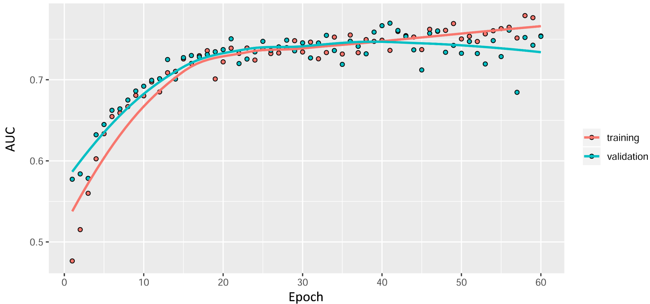
Fig. S1. Training phase of the CNN model. AUC, area under the receiver operating characteristic curve; CNN, convolutional neural network
