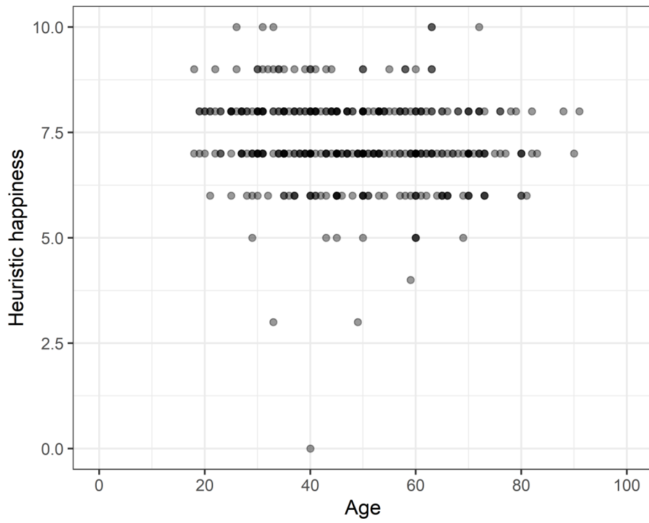
Fig. S1. Illustration of the squared effect of age on heuristic happiness.
