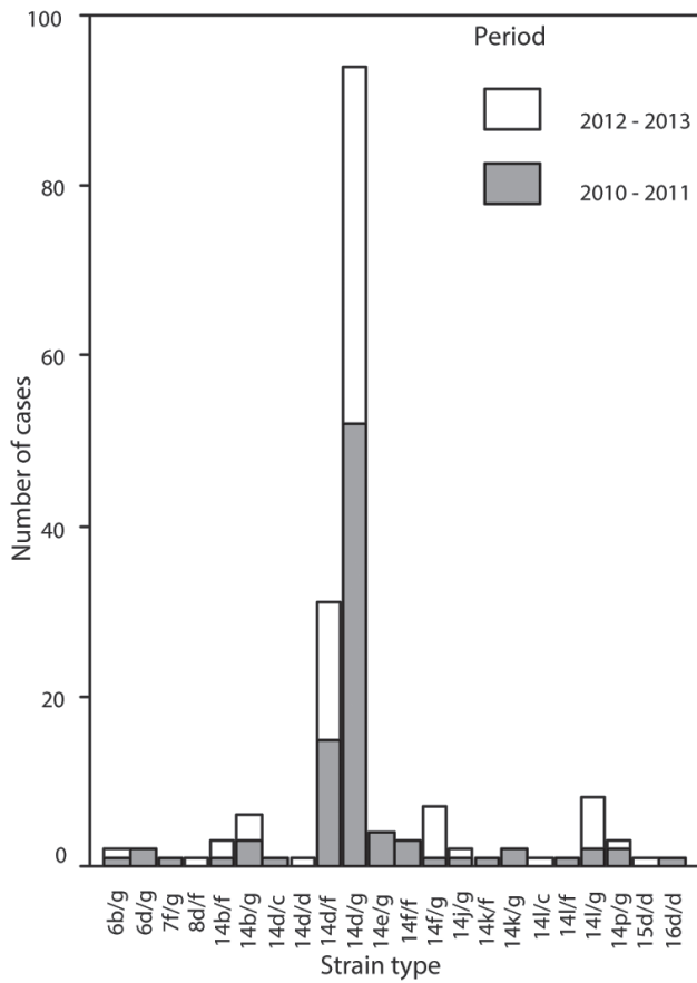
Fig. S1. Treponema pallidum strain type distribution in the periods 2010–2011 and 2012–2013.
