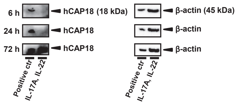
Fig. S1. hCAP18 protein (18 kDa) is detected in NHEK lysate at 72 h culture with IL-17A/IL-22. We used CAMP 293T Cell Transient Overexpression Lysate as positive control and \beta -actin (45 kDa) as internal control.
