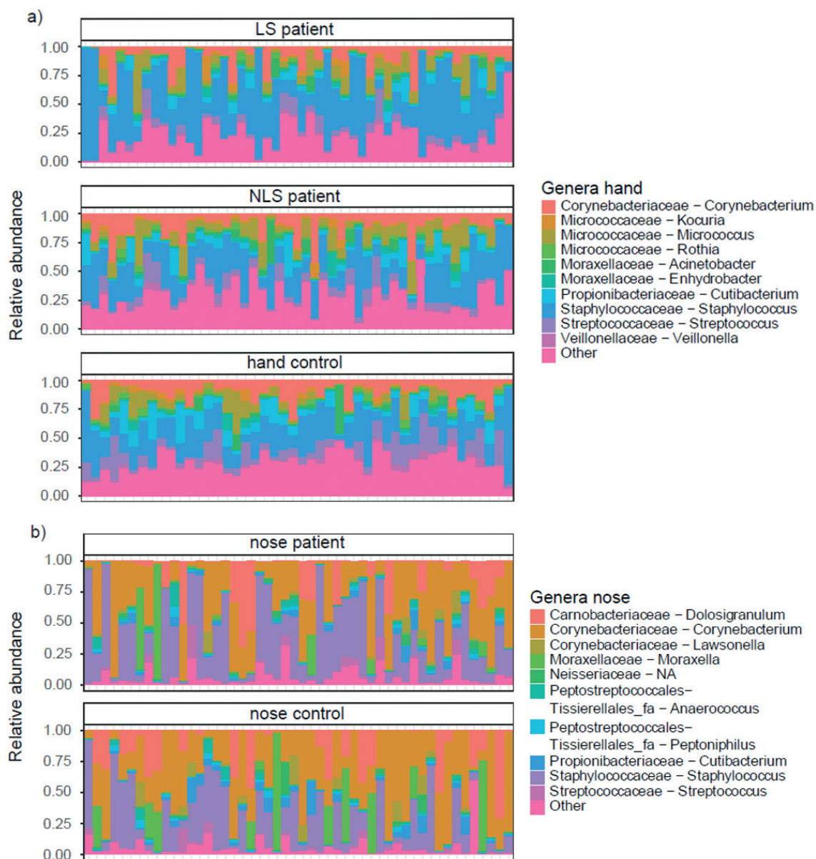
Fig. S2. Bacterial communities on the skin and in the nose of hand eczema (HE) patients and controls at baseline. The relative abundance of bacterial genera (a) on HE lesional skin, on HE non-lesional skin, on the hands of healthy controls, and (b) in the anterior nares of patients and healthy controls. The 10 overall most abundant genera are indicated in the plots.
