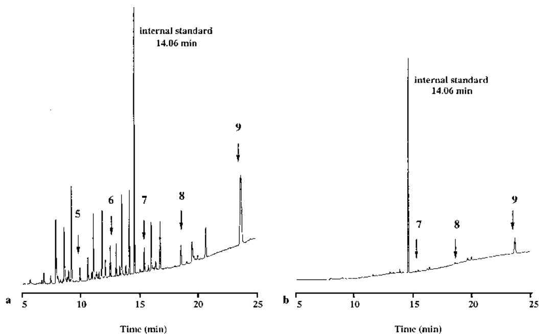
Fig. 12. GC chromatograms of the ethoxylated aldehydes identified in C 12 E 5 in (a) an undiluted sample stored and handled for 4.5 months at room temperature and in (b) a newly opened ampoule. The peaks are denoted with the same number as given to the corresponding synthetic reference compounds.
