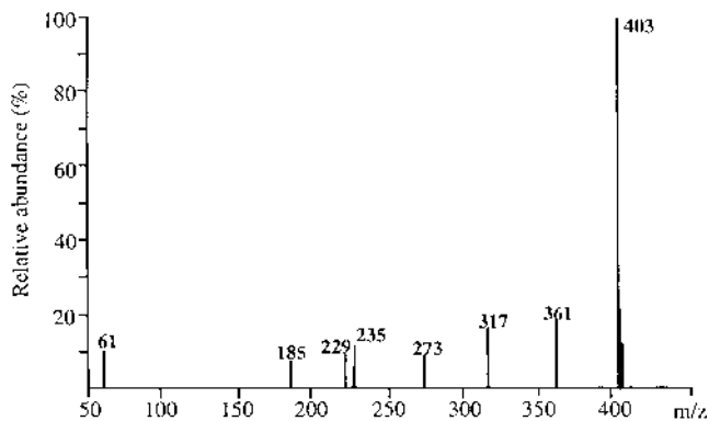
Fig. 13. MS-NICI spectrum of dodecyltetraoxyethyleneoxyacetaldehyde 9 , m/z 403=[M-1] - . The negative ions with a relative abundance >5% are shown in the spectrum.
