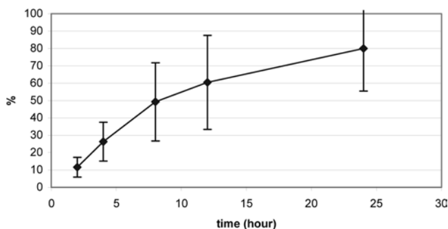
Fig. 2. Butorphanol release profile from liposome through full-thickness human skin by ultraviolet spectrophotometer (absorption at 280 nm, phosphate-buffered saline, 37°C). Using the full-thickness human skin sample, transdermal permeation measurement of the butorphanol liposome formulation was conducted in vitro with vertical diffusion Franz-cells. Samples were taken from the receiver at 2, 4, 8, 12 and 24 h after the start of the permeation experiment. As a control, full-thickness human skin without butorphanol liposome was used. The permeation of butorphanol through human skin shows that there was significant permeation at time-points 2, 4 and 8 h, and a steady state was achieved afterwards to 24 h ( \blacklozenge mean \pm SD, n=5 ).
