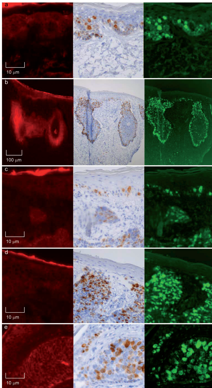
Fig. 2. Representative microscopic images of sections of superficial basal cell carcinoma (sBCC). Left image: protoporphyrin (PpIX) fluorescence distribution; middle and right images: Ki-67 staining. The middle image has been spectrally unmixed to show the distribution of Ki-67-positive cells. (a and b) Control lesions, 6 h after application of 20% 5-aminolaevulinic acid (ALA). (c–e) Sections 2 h after 20 Jcm -2 , and 6 h after application of 20% ALA. See detailed description in text.
