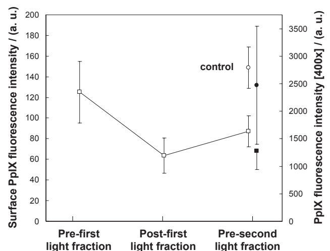
Fig. 3. Kinetics of surface protoporphyrin (PpIX) fluorescence intensity in superficial basal cell carcinoma (sBCC) during 5-aminolaevulinic acid-based photodynamic therapy (ALA-PDT) with a two-fold illumination scheme (open squares) delivering 20 \text{ J cm}^{-2} and the re-synthesis during the 2 h dark interval between light fractions and the PpIX fluorescence in un-illuminated control lesions (open circle – left axis). The corresponding mean microscopic PpIX fluorescence intensity (closed symbols – right axis) is shown for comparison. In all cases error bars represent standard deviations.
