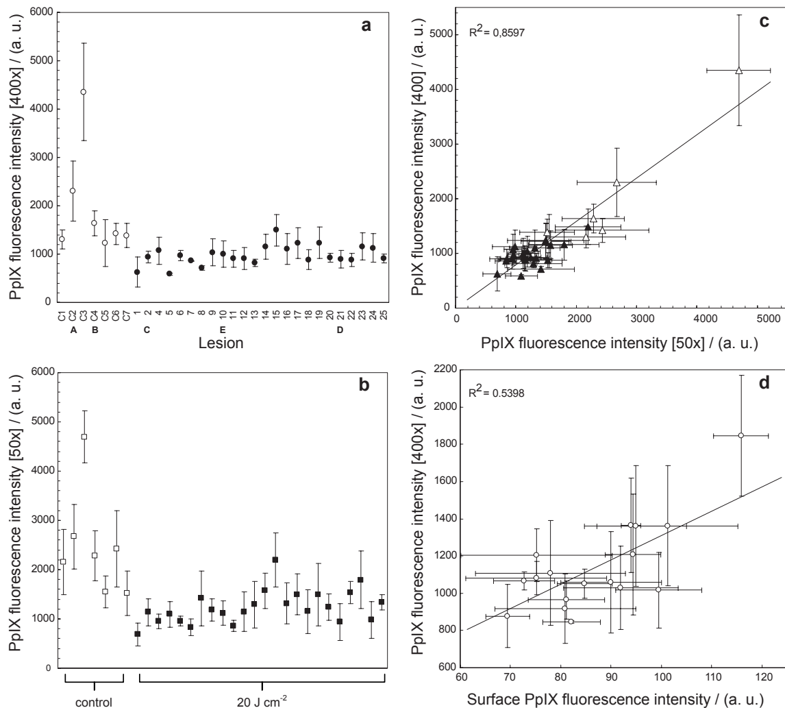
Fig. 1. Protoporphyrin (PpIX) fluorescence image analysis during 5-aminolaevulinic acid-based photodynamic therapy (ALA-PDT) of superficial basal cell carcinoma (sBCC), showing the mean microscopic fluorescence intensity measured using (a) 400 \times and (b) 50 \times magnification in control (c1–7) un-illuminated lesions 6 h after the application of 20% 5-aminolaevulinic acid (ALA) and in treated lesions (1–25) 2 h after 20 \text{J cm}^{-2} . (c) Correlation between the microscopic fluorescence intensity measured using 50 \times and 400 \times magnification. (d) Correlation between the surface and microscopic fluorescence intensity. In all cases error bars represent standard deviations. Unfilled symbols represent unilluminated lesions. Filled symbols represent illuminated lesions. a.u.: arbitrary units. (A–E refers to the lesions of Fig. 2).
