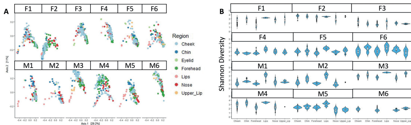
Fig. S2. (A) Principal coordinate analysis of Bray-Curtis dissimilarities coloured by region in each individual. (B) Shannon diversity of facial sites, grouped by individual.
