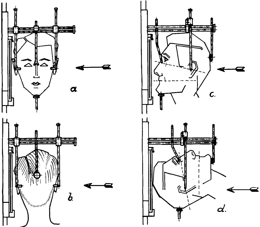
Fig. 3. Diagrammatic sketch of method of locating the skull when taking different X-ray projections, using the occlusion plane as a datum.
