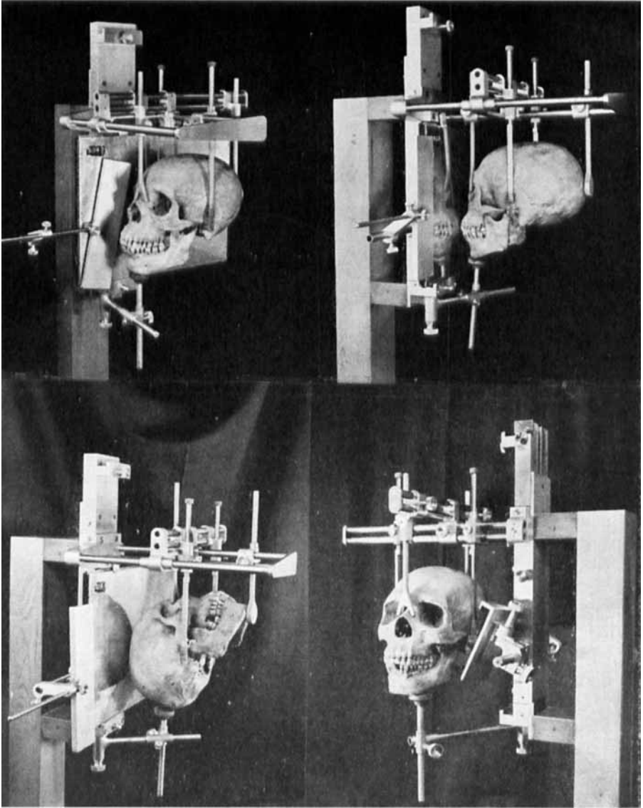
Fig. 1. Portable head holder for X-ray photography. The photographs illustrate how the head holder is used when taking lateral, frontal and basal exposures of the skull, as well as joint exposures.
