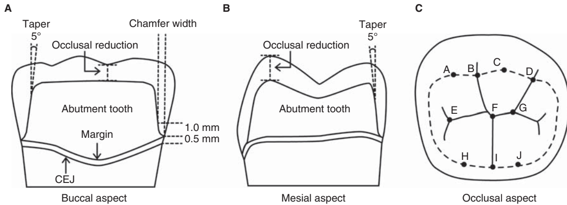
Figure 1. Schematic illustration of the abutment tooth 46 (A, B) and measurement points for occlusal reduction (C). Chamfer width was defined as the distance between the axial wall and the vertical line from the edge of finishing line at 1 mm above the margin. Occlusal reduction was measured as the vertical distance between the prepared and the non-prepared tooth models at 10 different points (A–J). The minimal occlusal thickness was obtained at B, F and I. CEJ, cement enamel junction.
