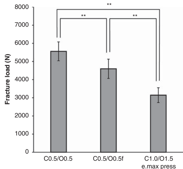
Figure 4. Comparison of fracture load of monolithic zirconia crown with reduced thickness (C0.5/O0.5 and C0.5/O0.5f) with that of lithium disilicate crown (C1.0/O1.5e.max press). Each value represents the mean with SD ( n=6 ).
