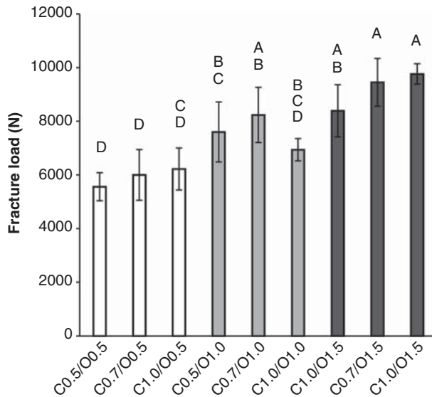
Figure 3. Fracture load of the monolithic zirconia crowns tested. Each value represents the mean with SD ( n=6 ). Different letters above the columns show significant differences ( p < 0.01 ) except for the difference between C0.7/O0.5 and C0.5/O1.0 ( p < 0.05 ).
