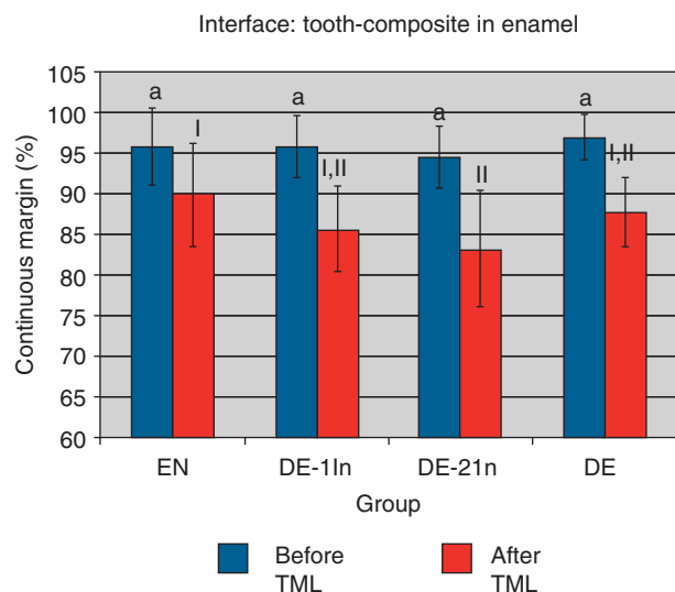
Figure 2. Continuous margins in enamel of the interface: tooth-luting composite. Percentages (mean \pm SD) of continuous margins in the experimental groups EN, DE-1In, DE-2In and DE as determined before and after TML. Groups indicated with the same superscript letter were not statistically significantly different.
