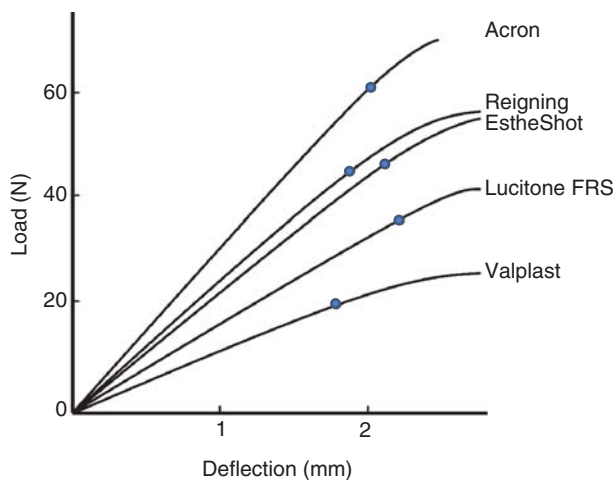
Figure 1. Load-deflection graphs of various denture base materials. The dots indicate the proportional limit.
