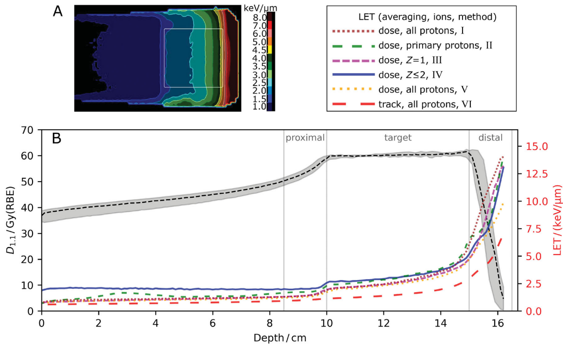
Figure 2. (A) Example of a linear energy transfer distribution (LET, dose-averaged, all protons), corresponding to the dose distribution in Figure 1(A). Line profiles of the six institutions along beam central axis are depicted in (B) for biologically equivalent dose with relative biological effectiveness of 1.1 ( D_{1.1} , gray, upper) and non-harmonized LET distributions (color-coded, lower). Median D_{1.1} (dashed, black) with minimum and maximum values (shaded area) and detailed depiction of LET line profiles for all six institutional non-harmonized LET calculations show inter-institutional variability. Roman numerals correspond to characteristic implementation parameters for LET calculation according to Table 2. Z: atomic charge.
