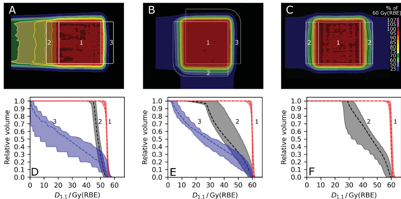
Figure 1. Dose distributions from one institution for a (A) single-field spread out Bragg-Peak, (B) perpendicular and (C) opposing field arrangement, displayed relative to the prescription dose of 60 Gy(RBE). (D), (E), (F) Dose-volume histograms (DVH) of the six institutions for each field arrangement (A), (B), (C), respectively, showing the median (dashed) and the interval from minimum to maximum DVH parameters (shaded area). A constant relative biological effectiveness (RBE) of 1.1 was applied to calculate the biologically equivalent dose ( D_{1.1} ). Regions of interest: (1) target volume, (2) proximal dose build-up region, (3) steep distal dose fall-off region.
