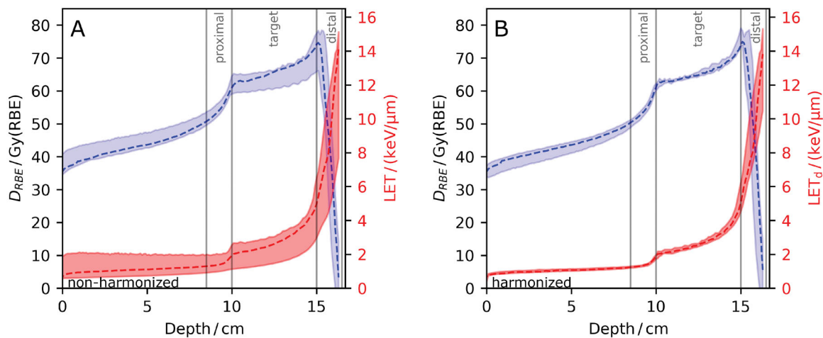
Figure 3. Line profiles from the six institutions along beam-central axis of the single-field spread-out Bragg peak for linear energy transfer (LET, red, lower) and for variable relative biological effectiveness (RBE)-weighted dose ( D_{RBE} , blue, upper) considering (A) non-harmonized LET and (B) harmonized LET d . D_{RBE} was calculated with the Wedenberg RBE model ( \alpha/\beta = 2 Gy). Median (dashed) D_{RBE} and LET are shown together with their minimum and maximum values (shaded area) showing inter-institutional variability. For definition of harmonized LET, please see section on Simulation of LET.
