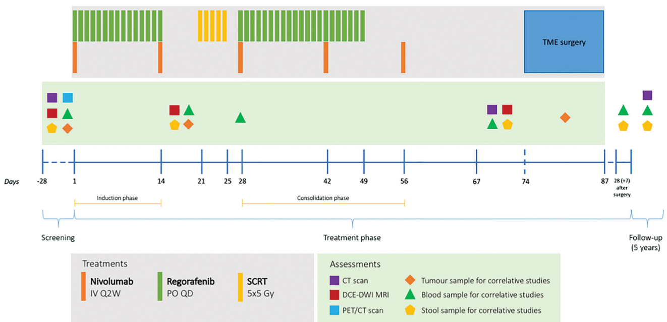
Figure 1. Study design.
