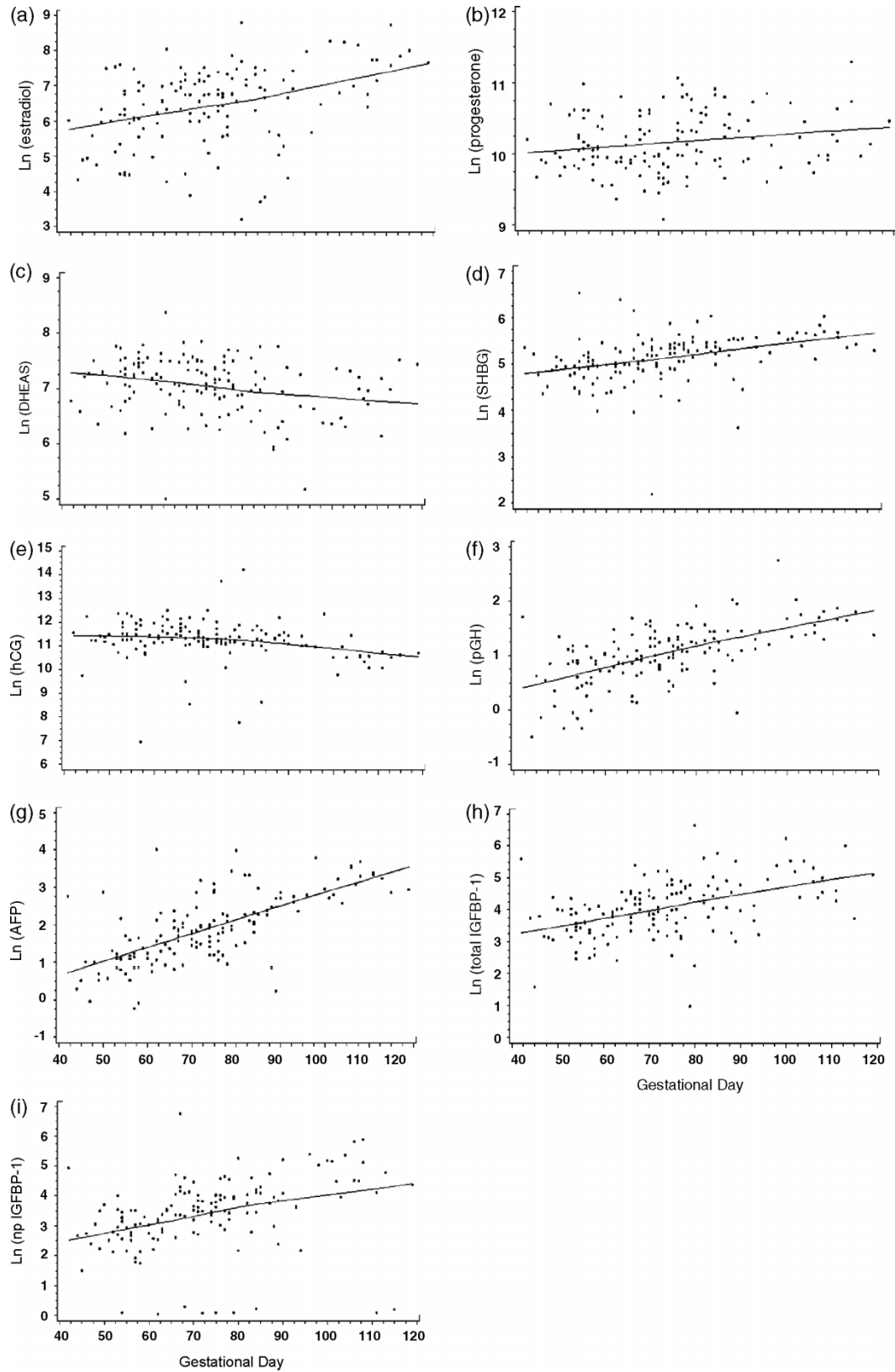
Figure 2. Variation of hormone levels by gestational day during early pregnancy in FMC biobank samples.* † a) estradiol ( p < 0.0001 ) ‡ , b) progesterone ( p < 0.01 ), c) DHEAS ( p < 0.002 ), d) SHBG ( p < 0.0001 ), e) hCG ( p < 0.0001 ), f) pGH ( p < 0.0001 ), g) AFP ( p < 0.0001 ), h) total IGFBP-1 ( p < 0.0001 ), i) np IGFBP-1 ( p < 0.0001 ). *Hormone levels presented on logarithmic scale. † Figures fitted using the local regression model. ‡ P-values (Spearman's ranked correlation analysis).
