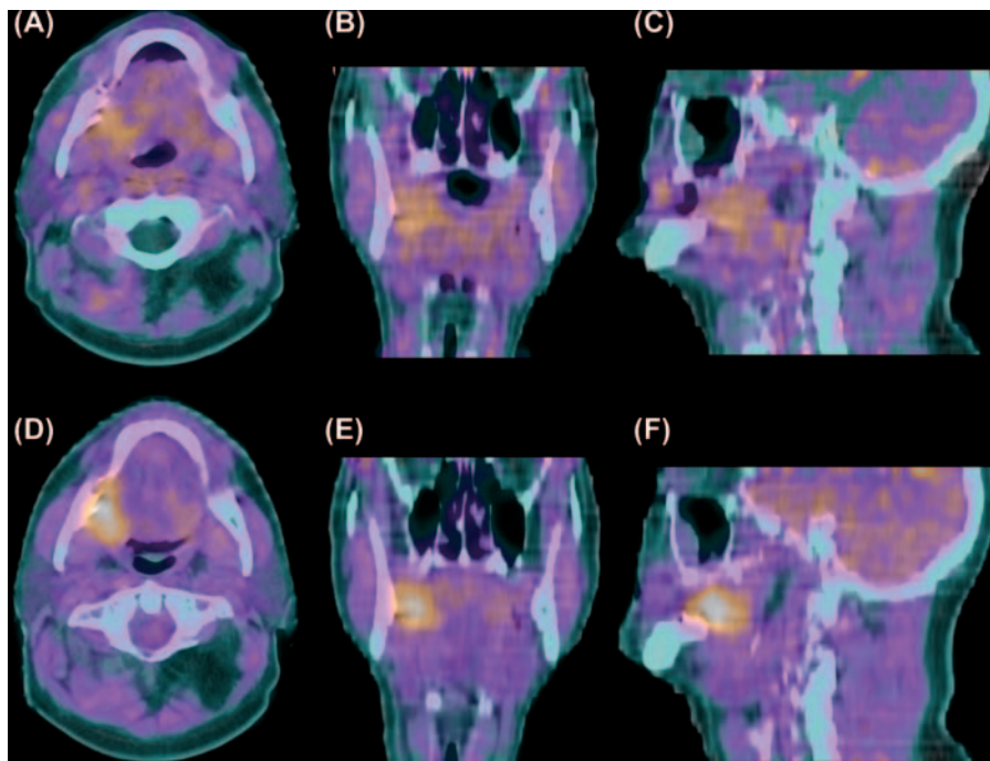
Figure 1. ^{18}\text{F} -FMISO PET-CT scan of a cT4N0M0 oral cavity tumor 30 min after injection with diffuse uptake in tumor and normal tissues (A–C) and 3 hours after injection with specific tumor retention (D–F). Transversal (A + D), coronal (B + E) and sagittal (C + F) planes.
