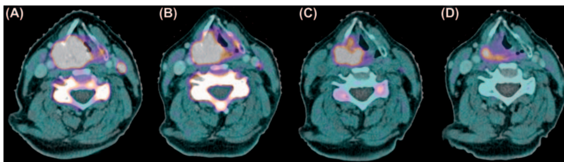
Figure 2. ^{18}\text{F} -FLT PET-CT scans of a patient with a cT4N2M0 hypopharyngeal tumor before therapy (A), after induction cetuximab (B), after 1 week of radiotherapy (two doses of cetuximab, 10 Gy) (C) and after 3 weeks of radiotherapy (four doses of cetuximab, 32 Gy) (D). Note the concurrent reduction in cervical vertebra marrow proliferation after start of radiotherapy.
