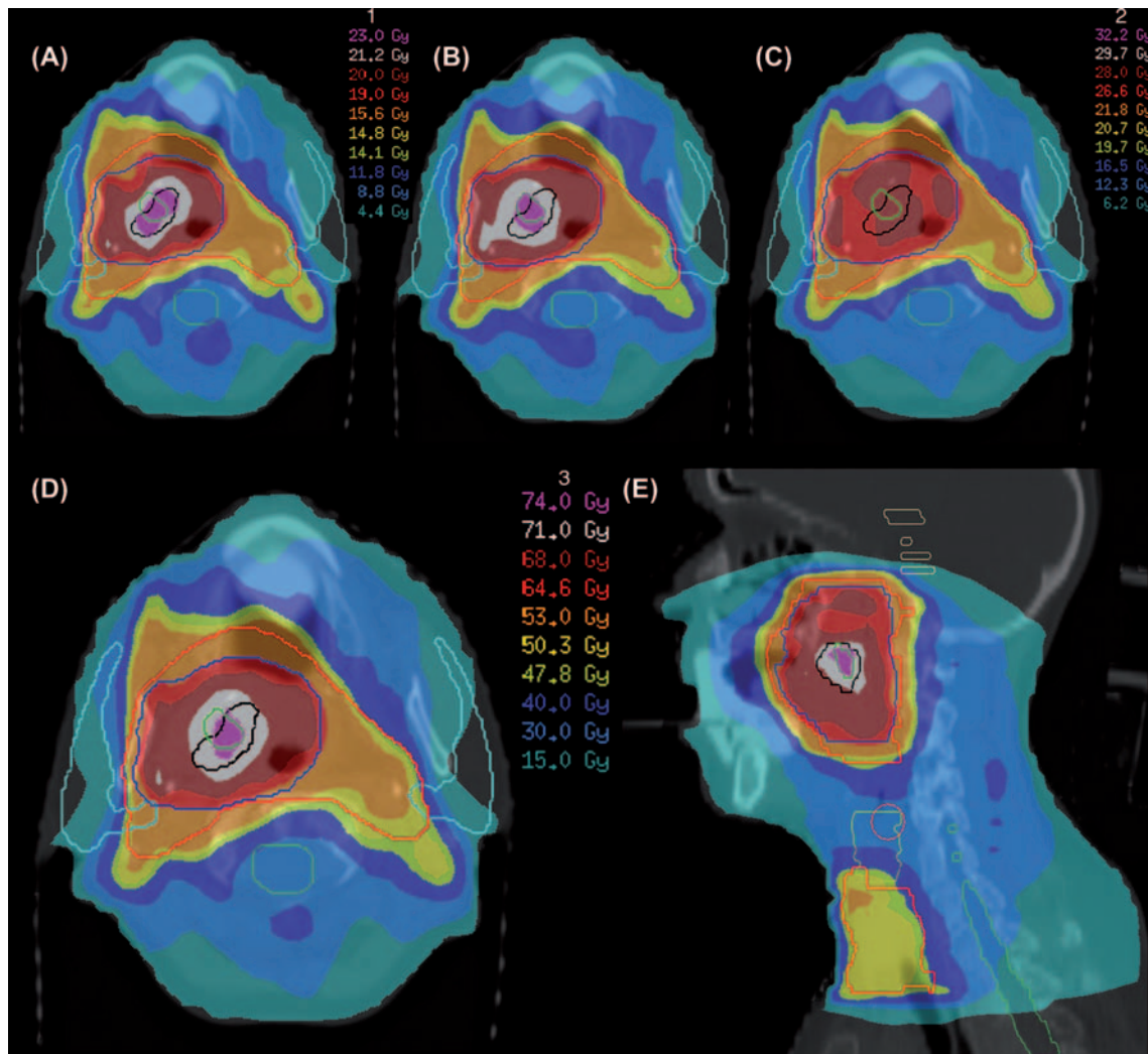
Figure 3. Dose-escalation to GTV_{80\%1} (as delineated using a cut-off of 80% of maximum tumor uptake signal in a ^{18}F -FLT PET-CT scan performed before start of radiotherapy) and GTV_{80\%2} (as delineated in a ^{18}F -FLT PET-CT scan performed after 1 week of radiotherapy) for a cT3N0M0 oropharyngeal tumor. Using IMRT with integrated simultaneous boost technique, total dose was 50.3 Gy to bilateral cervical lymph node regions (large planning target volume, red) and 68 Gy to primary tumor (small planning target volume, blue); in 34 fractions. GTV_{80\%1} (black) and GTV_{80\%2} (green) were consecutively irradiated with 2.3 Gy for 10 fractions, resulting in a dose of 71 Gy in total and a dose of 74 Gy in the overlapping region. (A and B) Dose distributions for first 2 weeks of treatment (A) and weeks 3 and 4 (B). (C) Dose distribution for remaining 14 fractions without dose-escalation. (D and E) Dose distributions of total treatment plan in transverse (D) and sagittal (E) planes. Parotid glands are delineated in sky blue and spinal cord in green. This figure was originally published in JNM. Troost EG, Bussink J, Hoffmann AL, Boerman OC, Oyen WJ, Kaanders JH. ^{18}F -FLT PET/CT for early response monitoring and dose-escalation in oropharyngeal tumors. J Nucl Med 2010;51:866–74. (©) by the Society of Nuclear Medicine and Molecular Imaging, Inc.
