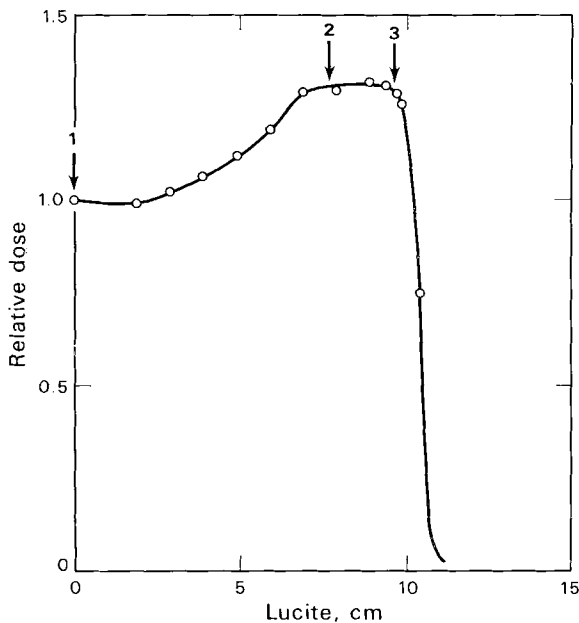
Fig. 1. Modified depth-dose distribution of a 910 McV helium ion beam used with a ridge filter, showing the three exposure positions.
