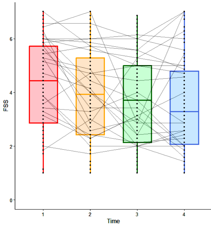
Fig. SI. Distribution of fatigue severity over time
