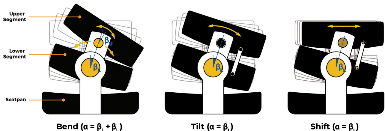
Fig. 2. The behaviour of the modular backrest could be configured to 3 different modes without the need for participants to transfer out of the wheelchair.
